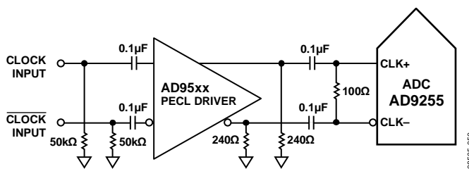
Figure 77. Differential PECL Sample Clock (Up to Rated Sample Rate)
