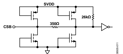
Figure 60. Equivalent CSB Input Circuit
