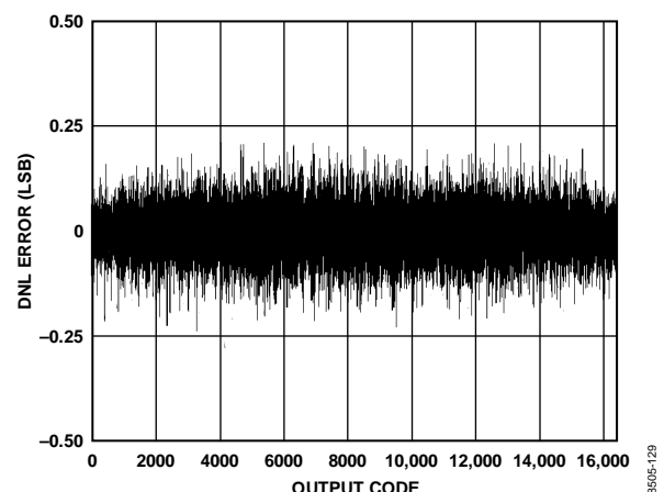
Figure 29. AD9255-105 DNL with f_{IN} = 12.5 MHz
