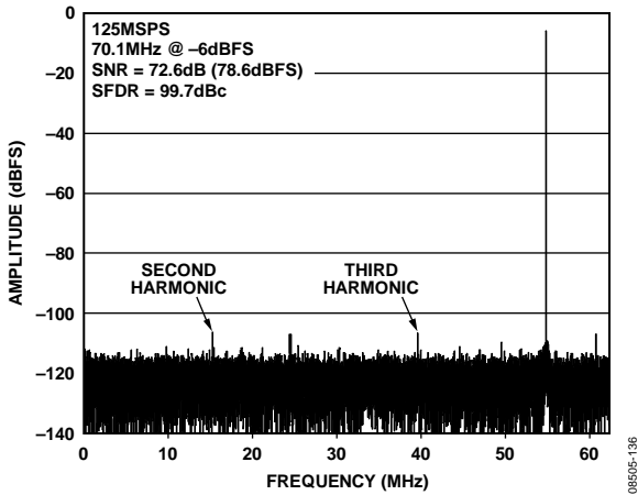
Figure 36. AD9255-125 Single-Tone FFT with f_{IN} = 70.1 MHz @ -6 dBFS with Dither Enabled
