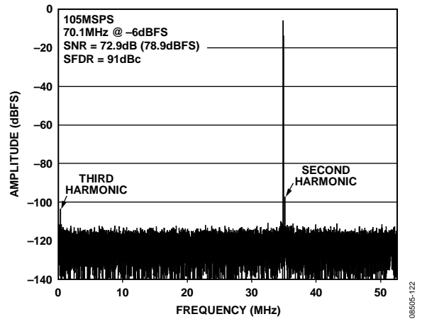
Figure 22. AD9255-105 Single-Tone FFT with f_{IN} = 70.1 MHz @ -6 dBFS with Dither Enabled
