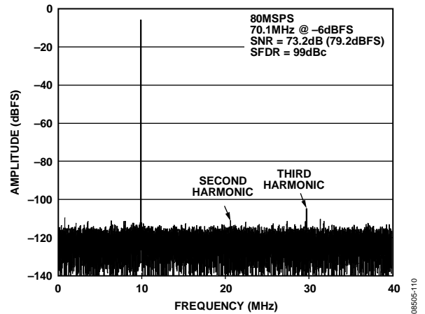
Figure 10. AD9255-80 Single-Tone FFT with f_{IN} = 70.1 MHz @ -6 dBFS with Dither Enabled
