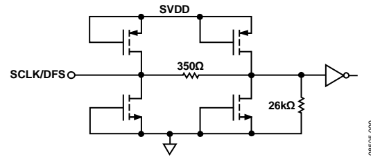
Figure 59. Equivalent SCLK/DFS Input Circuit
