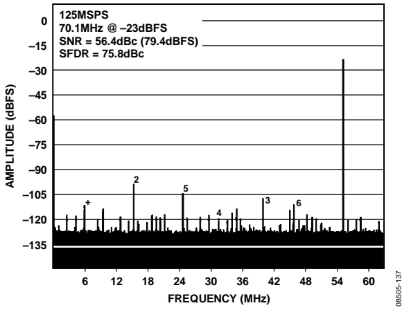
Figure 37. AD9255-125 Single-Tone FFT with f_{IN} = 70.1 MHz @ -23 dBFS with Dither Disabled, 1M Sample
