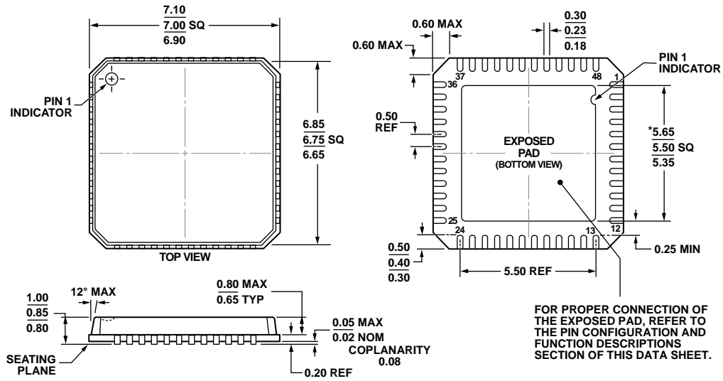
*COMPLIANT TO JEDEC STANDARDS MO-220-VKGD-2 WITH EXCEPTION TO EXPOSED PAD DIMENSION. Figure 85. 48-Lead Lead Frame Chip Scale Package [LFCSP_VQ] 7 mm × 7 mm Body, Very Thin Quad (CP-48-8) Dimensions shown in millimeters
